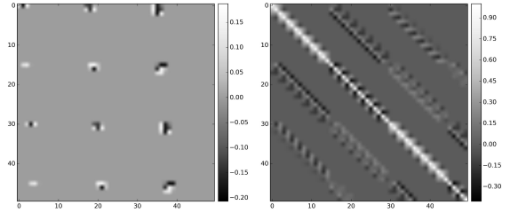
Figure 5: learned sparse weights W for the last SVM layer in Tiled CNN (left) and its orthogonality constraint by WW^T = I (right).
